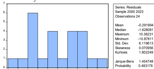
Figure 13 Normality Test
